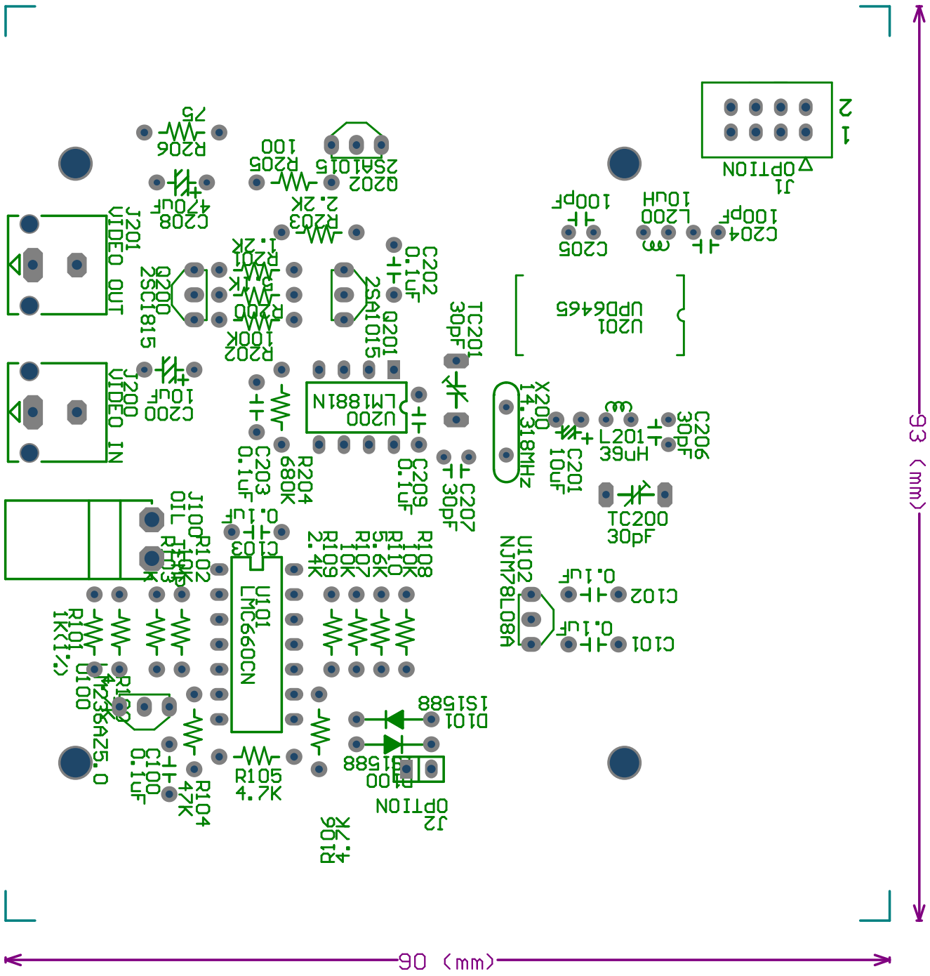
PCB Sanhayato 1/2 42K, Chassis TAKACHI SU-140
