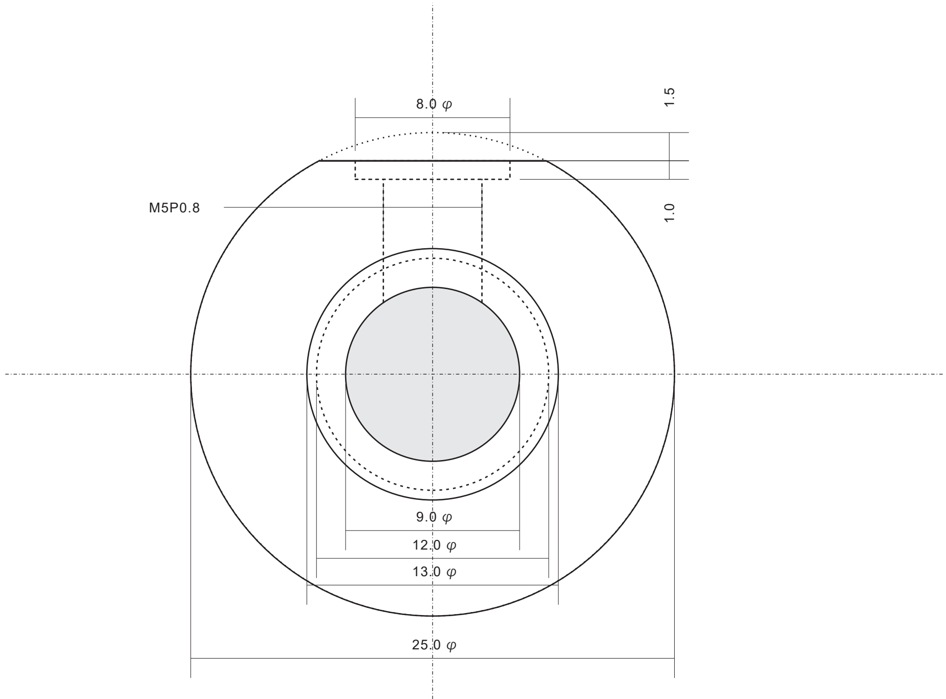
3Way joint LEFT VIEW
