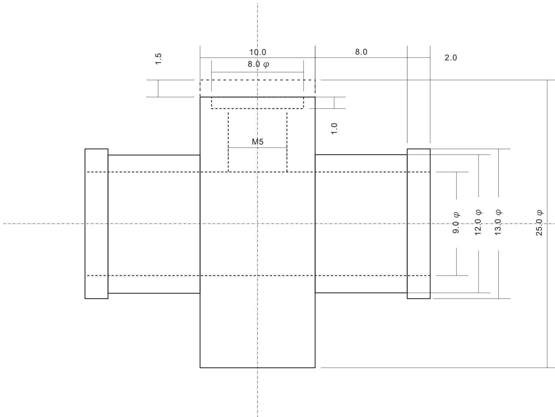
3Way joint FRONT VIEW
